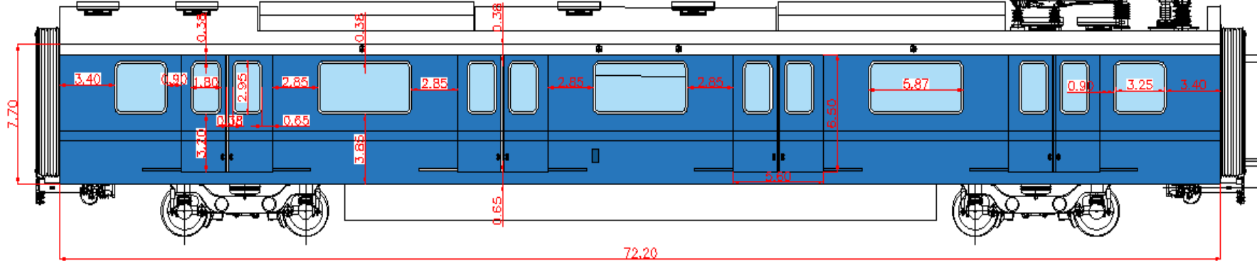
T/M CAR (Middle Car) - 866"Length x 94" Height In (84"+10"Top strip)
