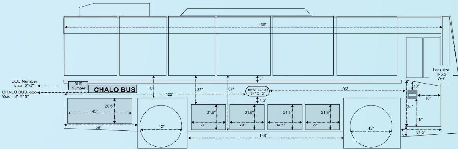
JBM BUS -RIGHT SIDE SIZES
