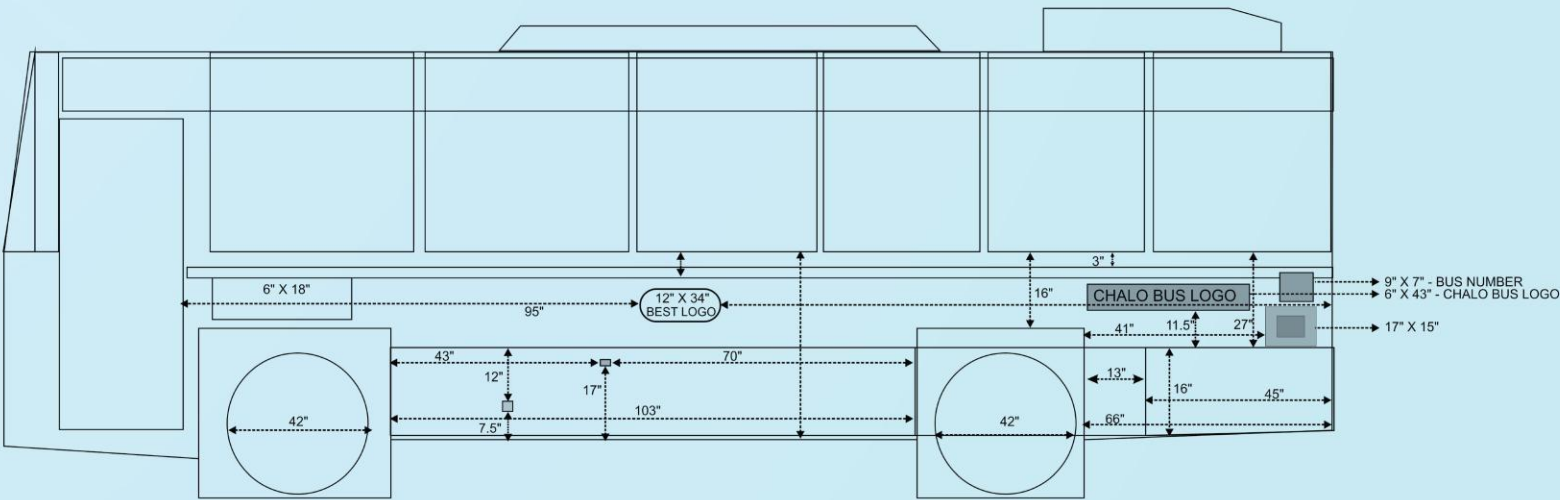
JBM BUS -LEFT SIDE SIZES
