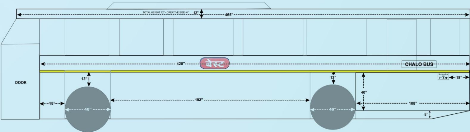
BEST- LEFT SIDE-SWITCH -12 MTR
